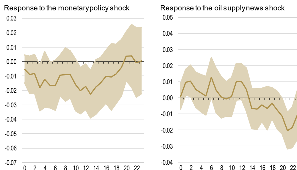
Figure 4: Impulse responses of the ISMI to exogenous shocks
