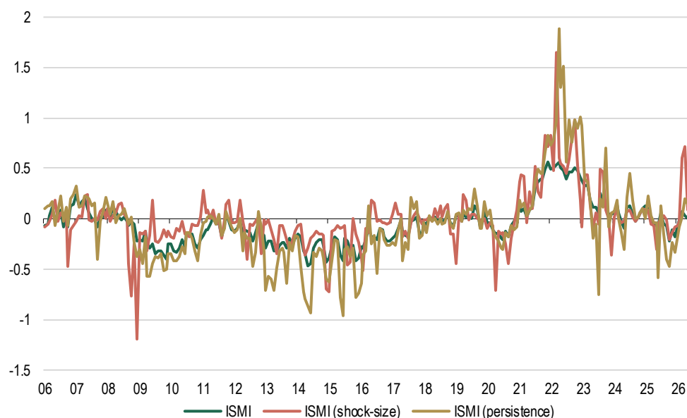
Figure 9: Monthly ISMI along with shock-size and inflation persistence adjusted counterparts
