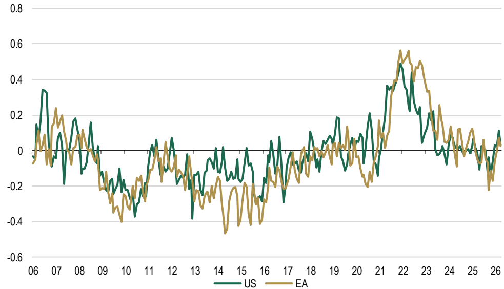
Figure 3: Comparison between the ISMI for the euro area and the US
