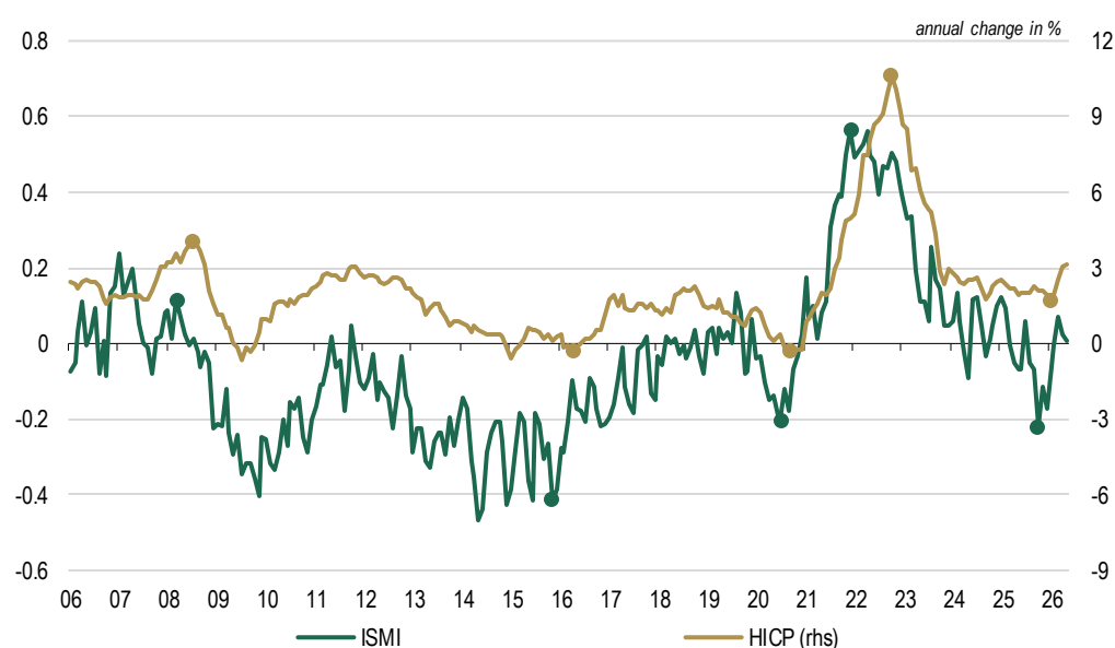
Figure 5: Turning points of the ISMI and headline inflation
