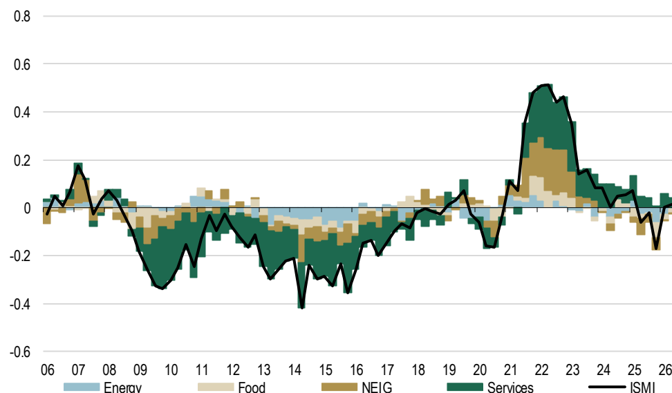
Figure 2: Quarterly decomposition of the ISMI according to the main inflation components
