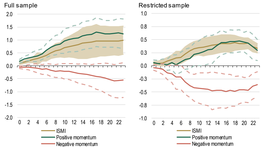
Figure 6: Dynamic changes of the price level associated with the ISMI and momentum shares
